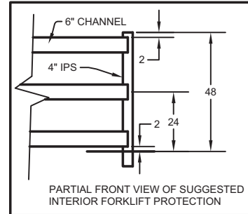
BOLLARD SECTION (SUGGESTED)
