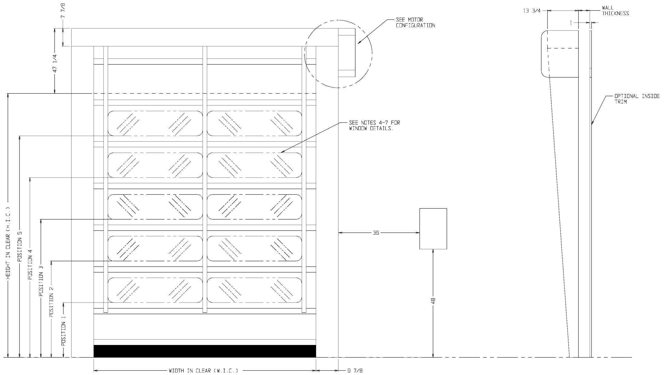
VERTICAL SECTION
